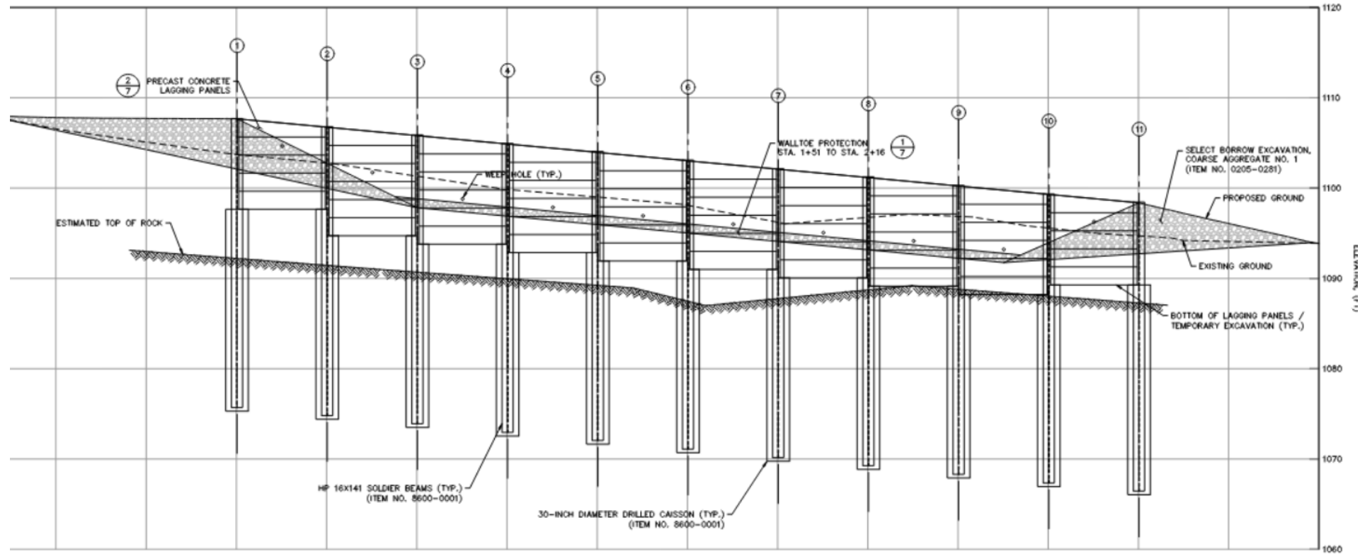
RETAINING WALL ELEVATION
